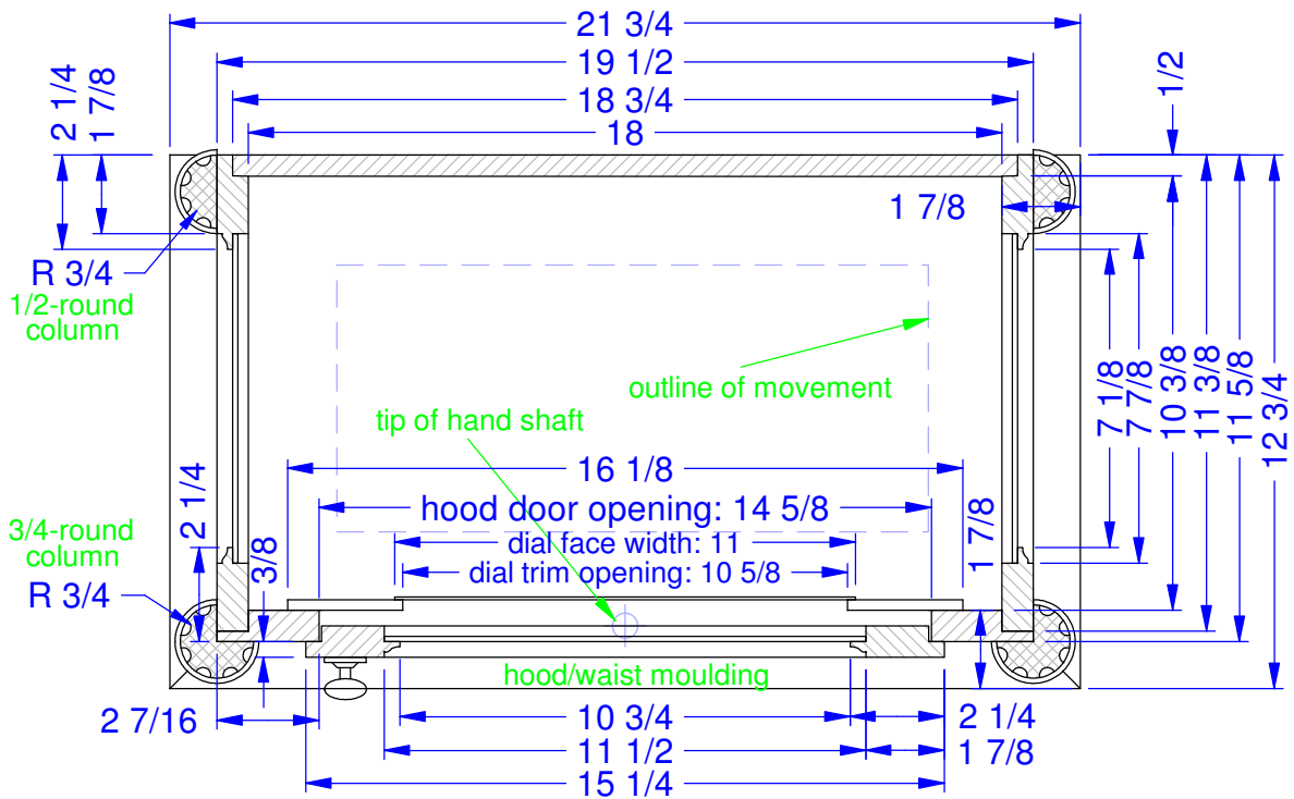
section C-C (hood)
