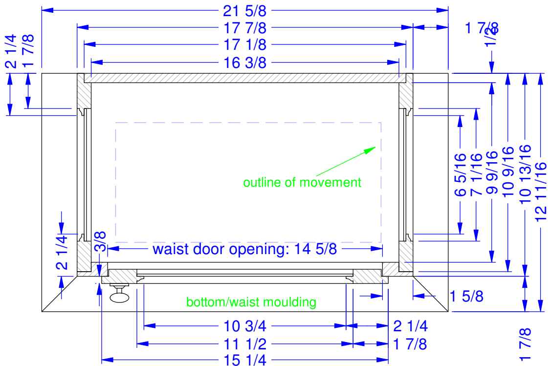
section D-D (waist)
