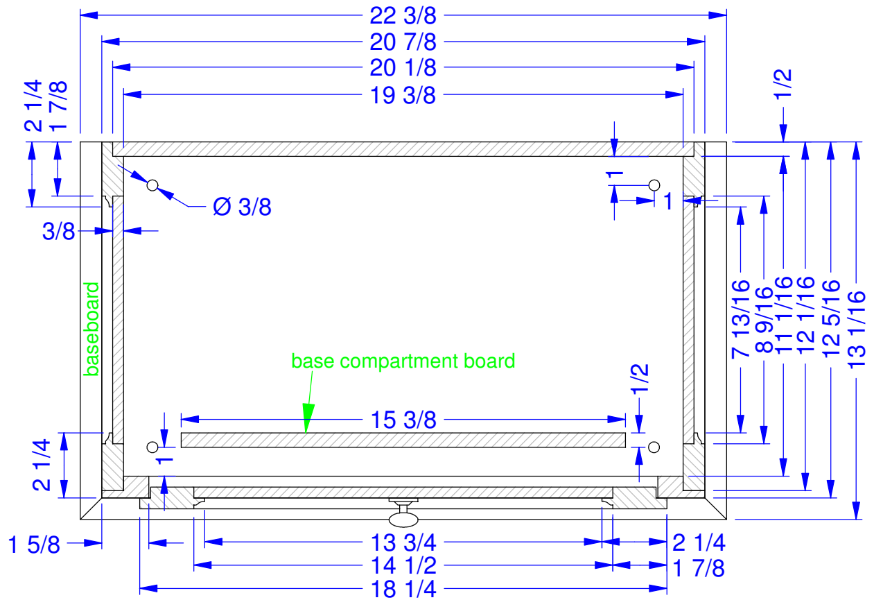
section E-E (base)
